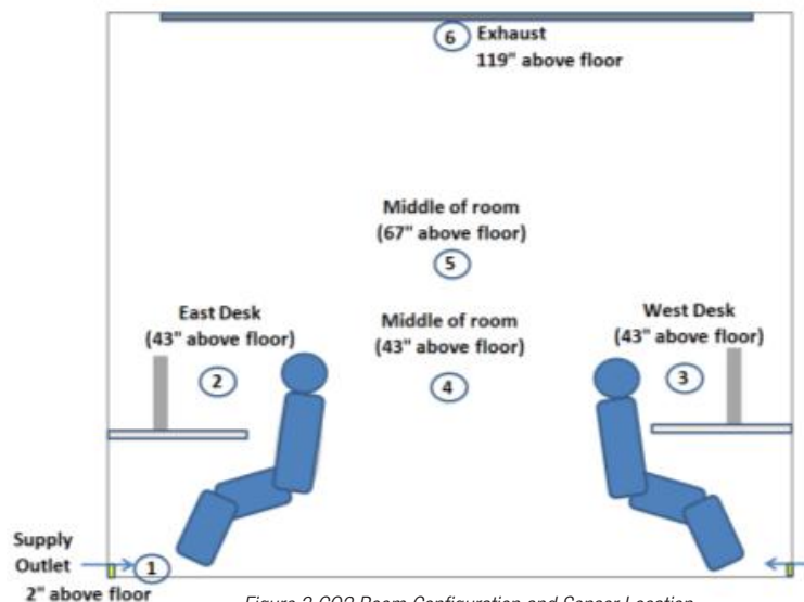
Figure 3 CO2 Room Configuration and Sensor Location
