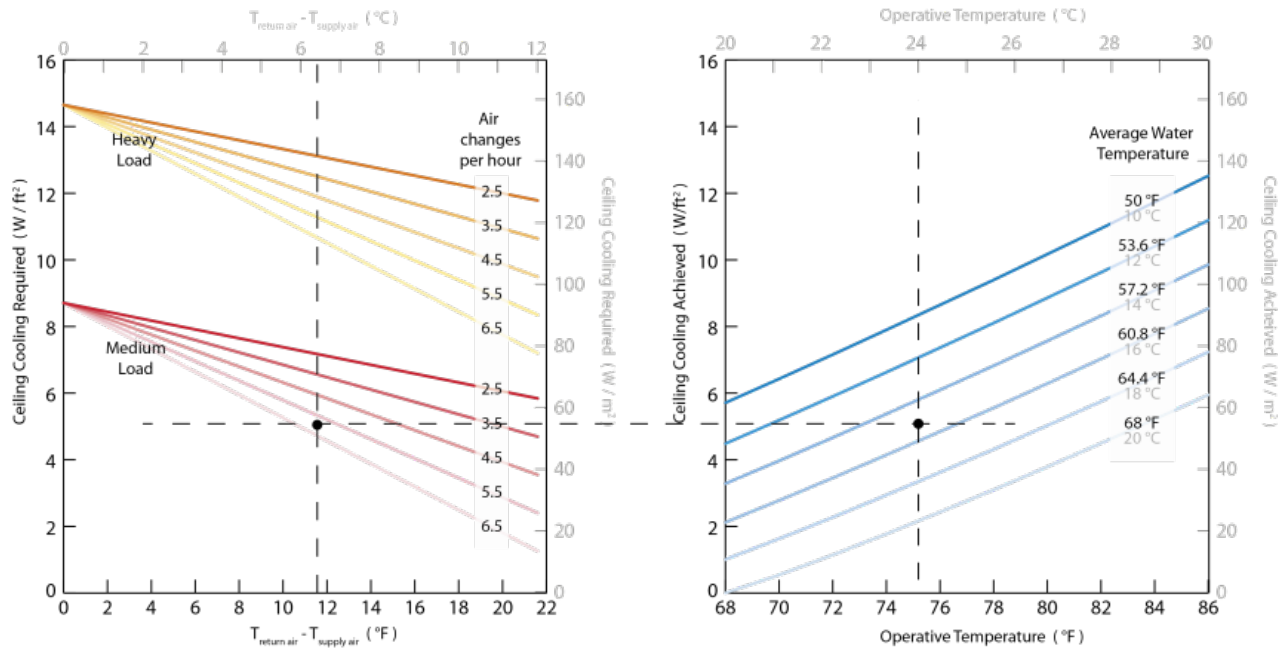
Figure 1 Cooling Nomogram
