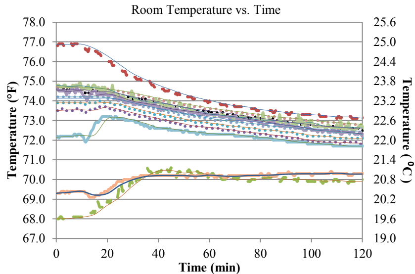
Figure 4 Decay in room temperature after the removal of the occupant and equipment loads
