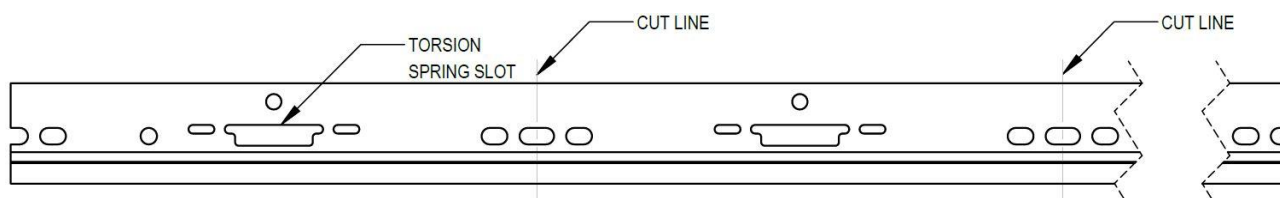
Figure 30 – Runner cut line for onsite cutting
