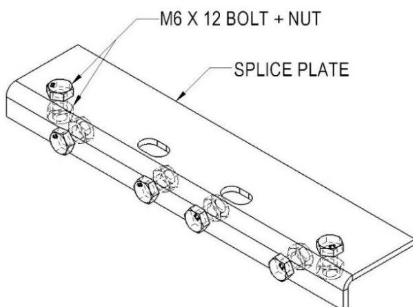
Figure 4 – Splice Plate
