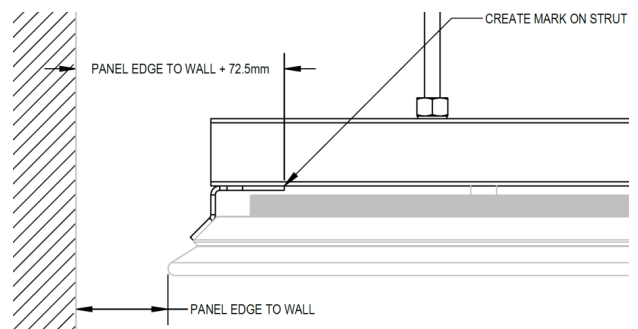
Figure 15 – Runner positioning in X-direction – 1st row
