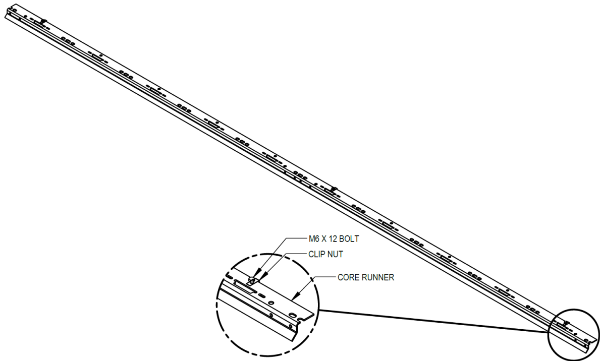
Figure 3 – Core Runner
