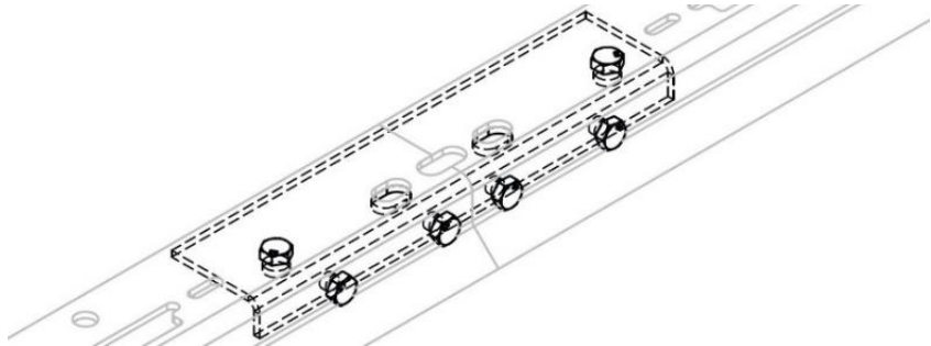
Figure 24 – Iso view of Core Runner and Splice Plate
