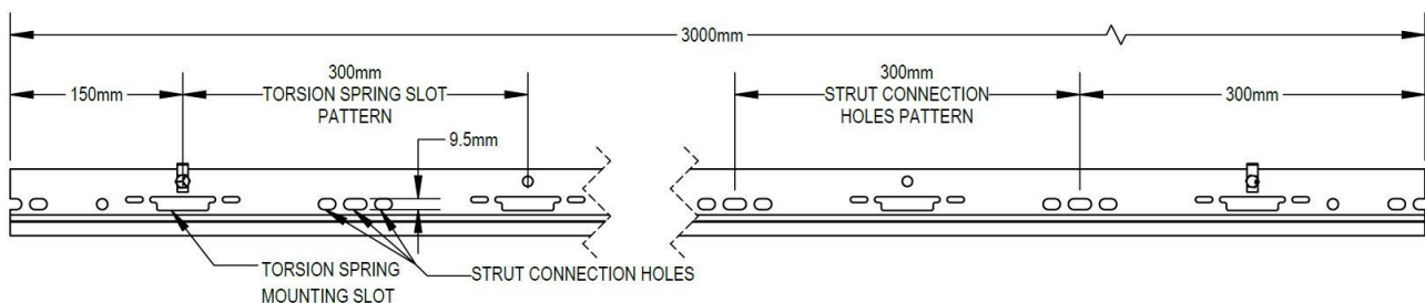
Figure 12 – Runner dimensions
