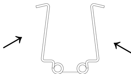
FIGURE 16: COMPRESS TORSION SPRING LEGS TOGETHER
