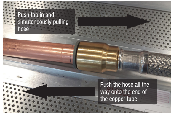
FIGURE 15: HOSE ENGAGEMENT
