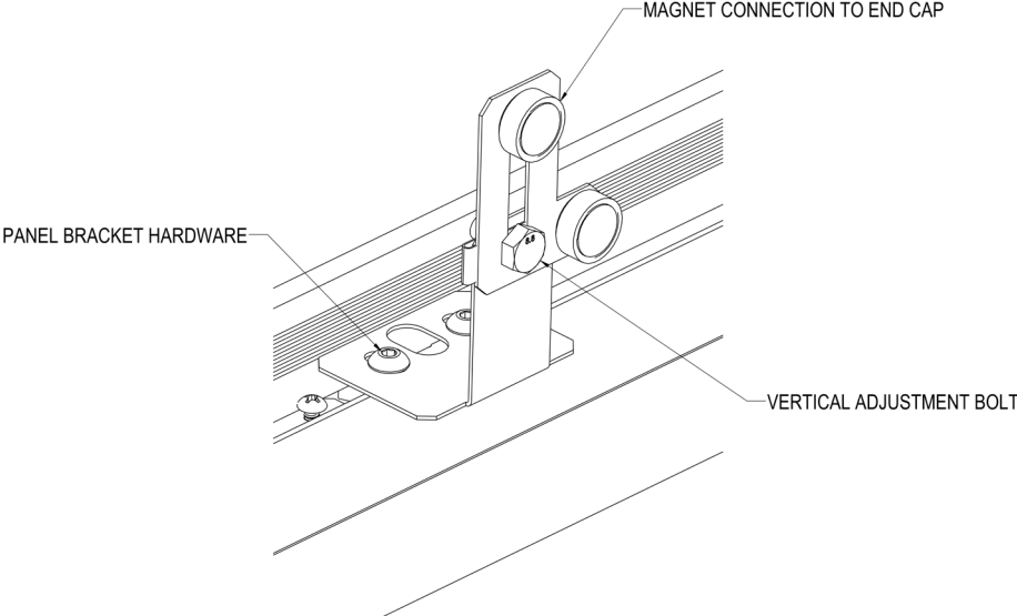
FIGURE 24: END CAP BRACKET CORE MOUNTED
