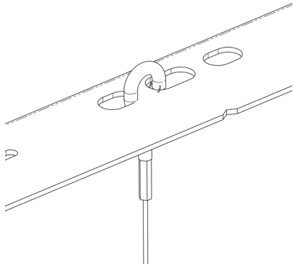
FIGURE 12: ACCESS CABLE CONNECTED TO CORE RUNNER
