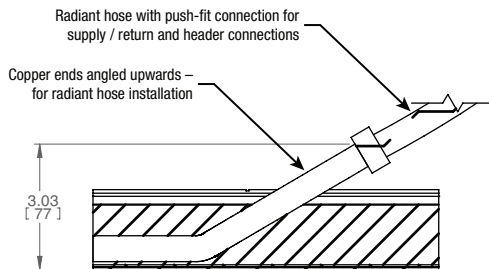
FIGURE 14: HOSE INSTALLATION
