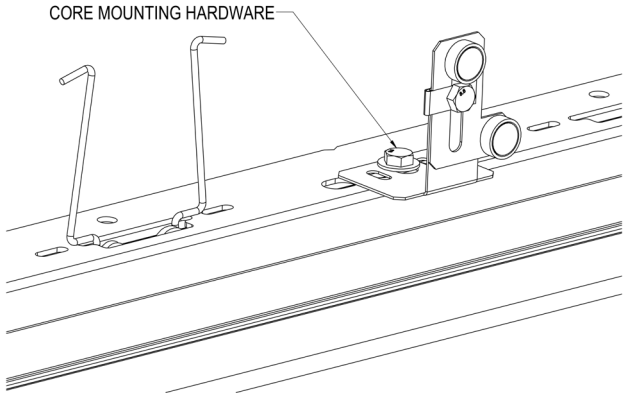
FIGURE 24: END CAP BRACKET CORE MOUNTED
