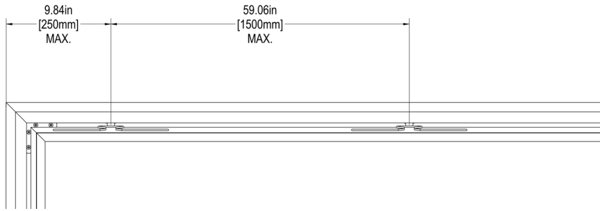
FIGURE 4: MAXIMUM DISTANCES BETWEEN TORSION SPRINGS
