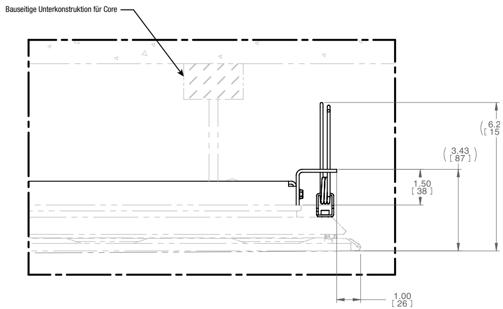
ABBILDUNG 18: WEAVE PANEEL IN FINALER MONTAGEPOSITION
