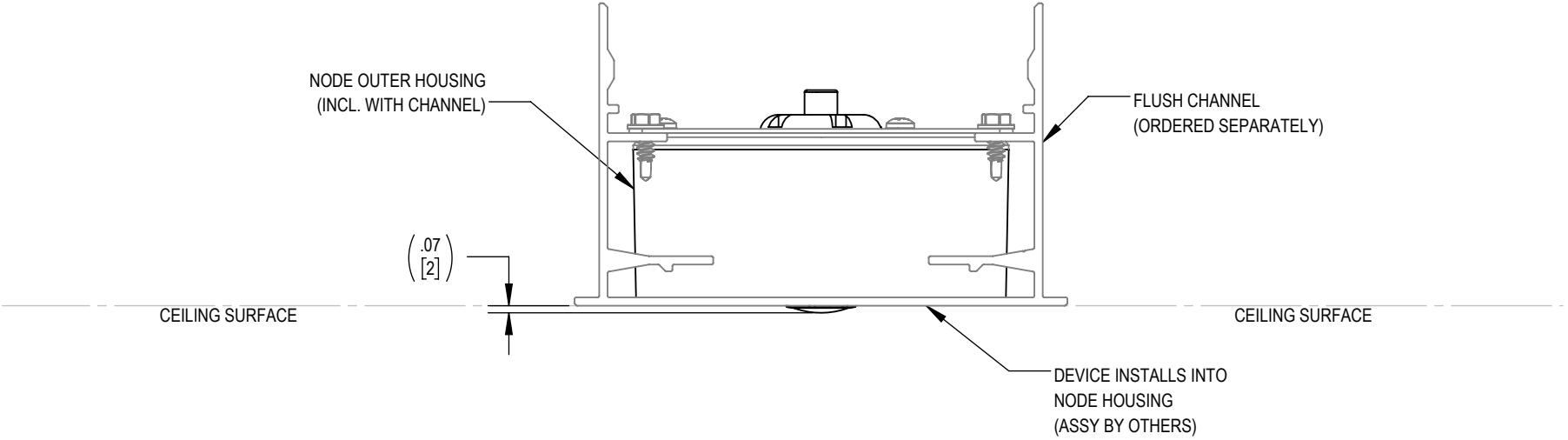
SIDE VIEW FLUSH CHANNEL
