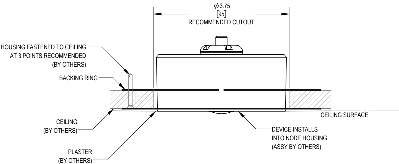
CEILING CROSS SECTION
