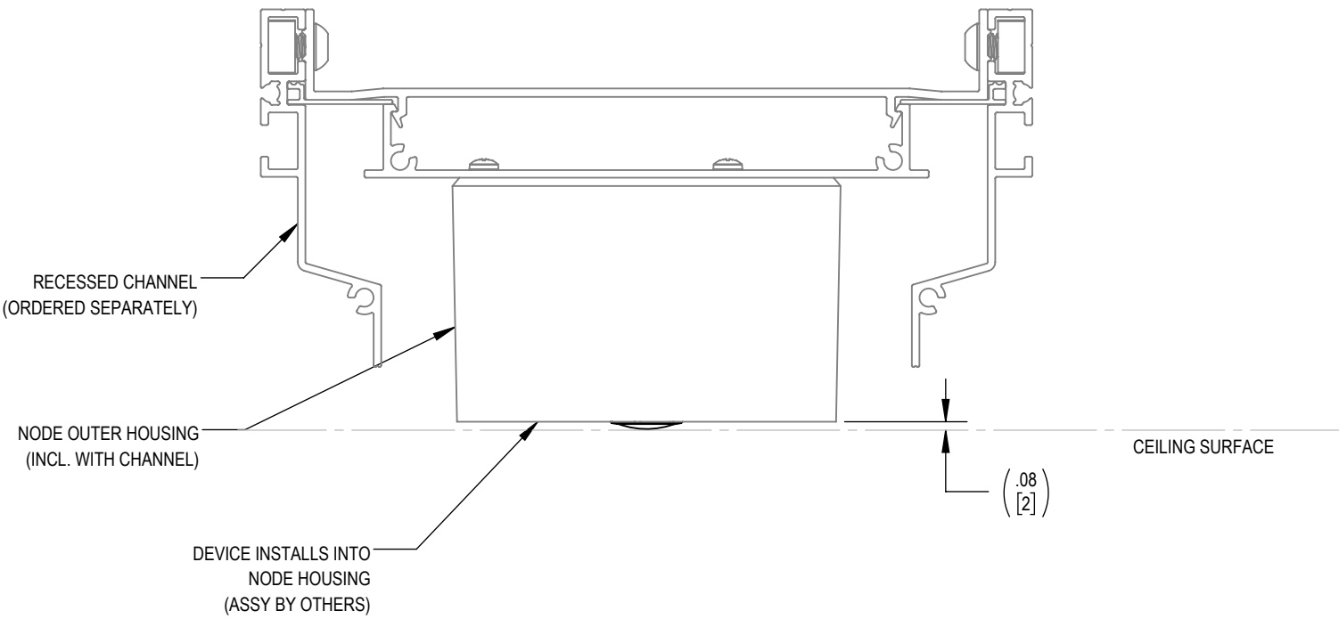
SIDE VIEW RECESSED CHANNEL
