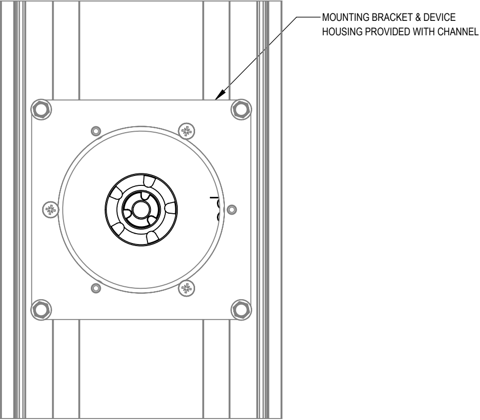
TOP VIEW FLUSH CHANNEL
