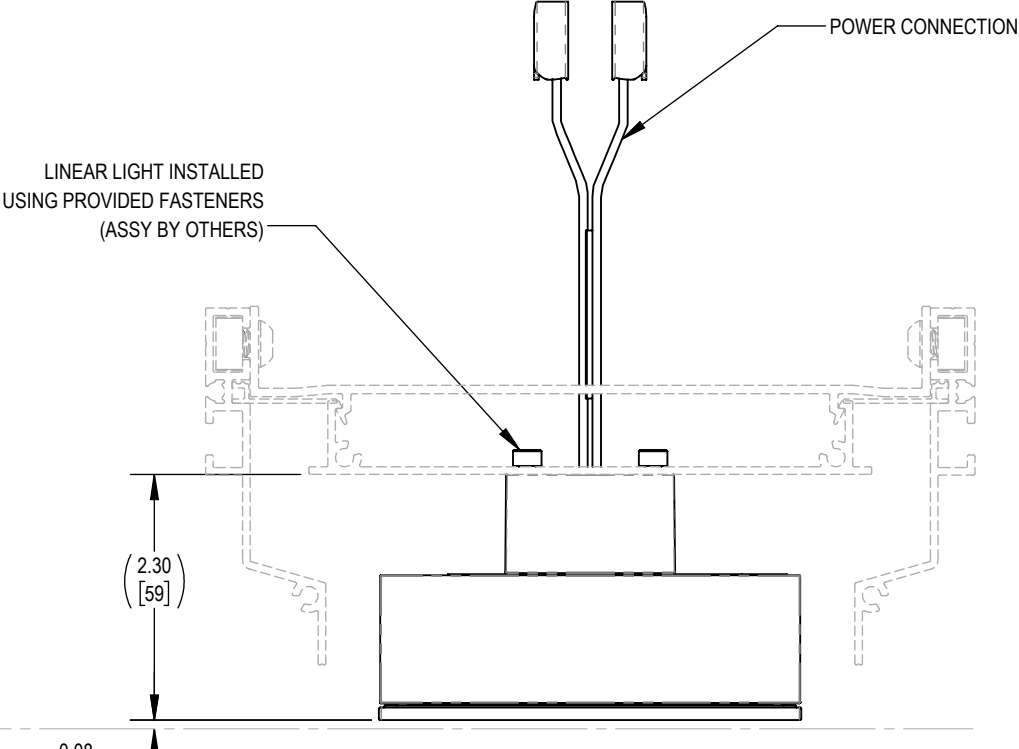
END VIEW RECESSED CHANNEL
