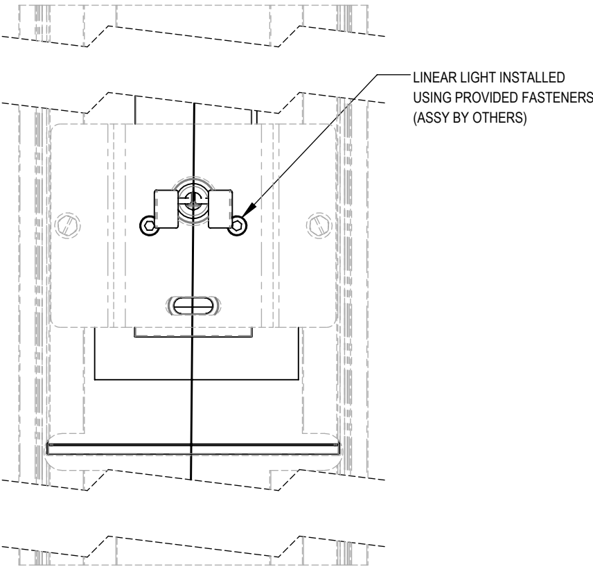
TOP VIEW FLUSH CHANNEL, MOUNTING BRACKET DETAILS
