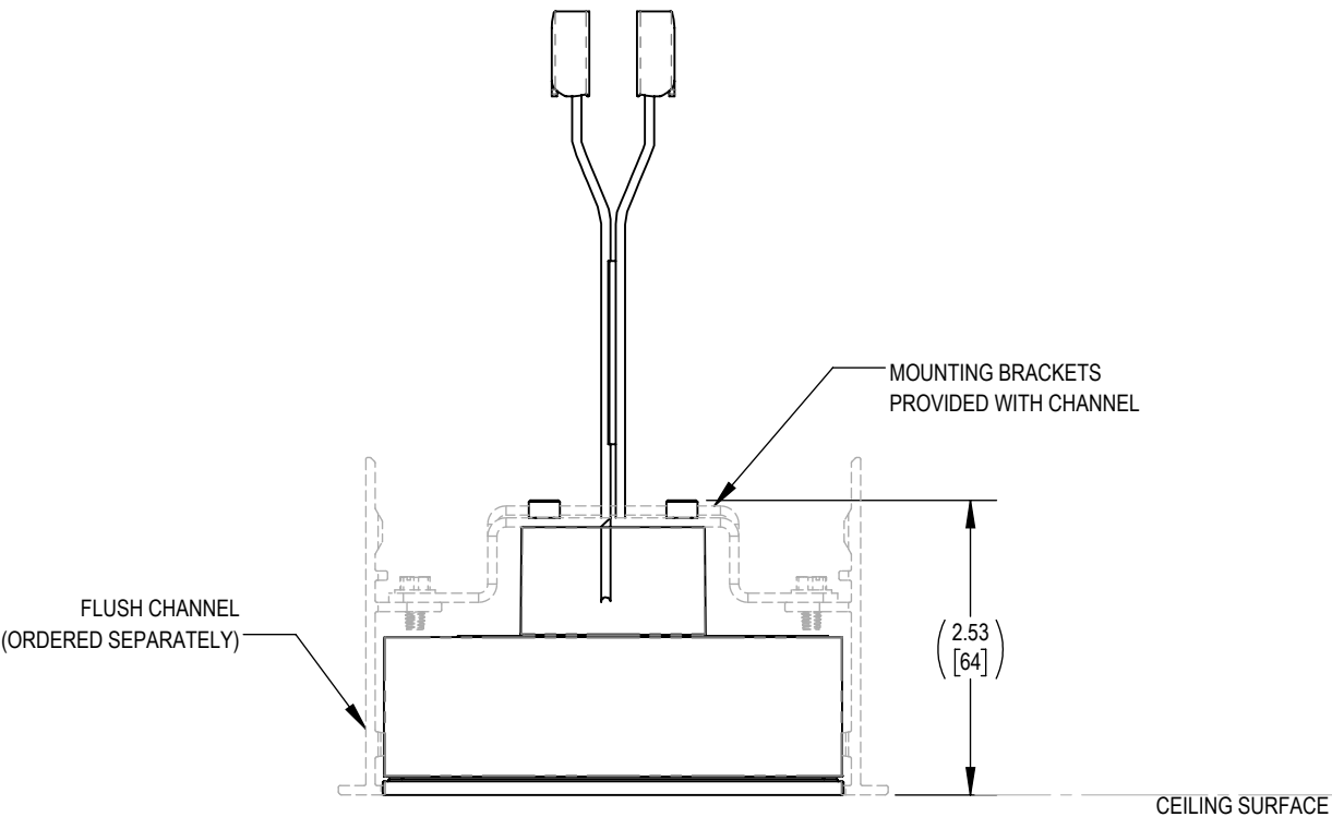
END VIEW FLUSH CHANNEL
