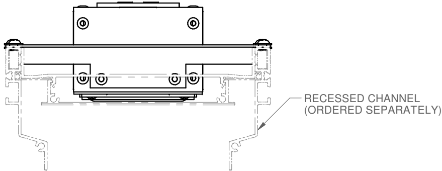
END VIEW RECESSED CHANNEL
